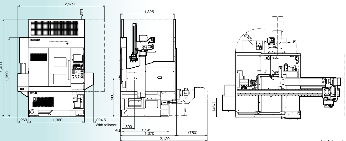
Gantry Loader type
