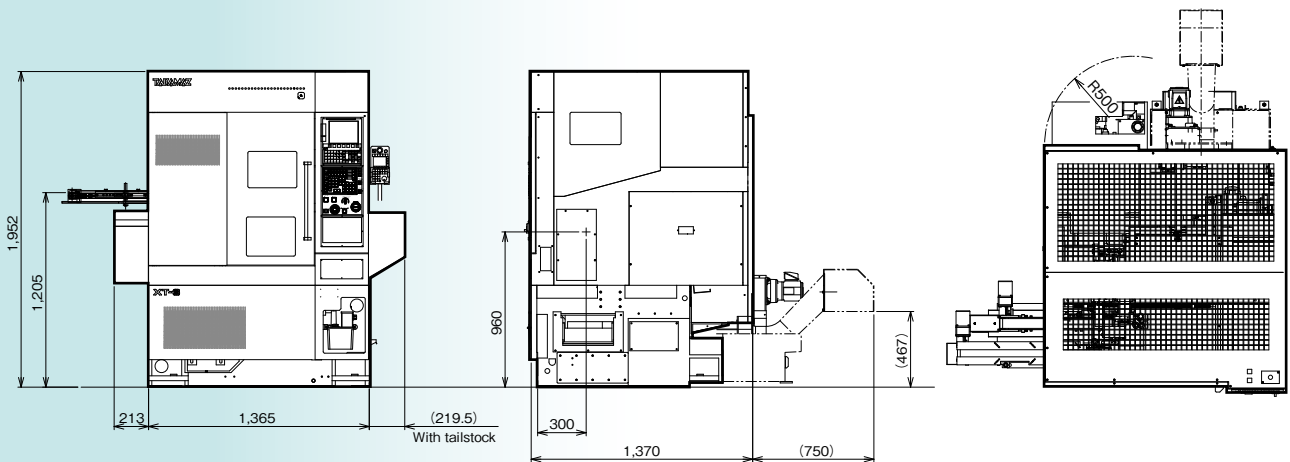
Compact Loader type
